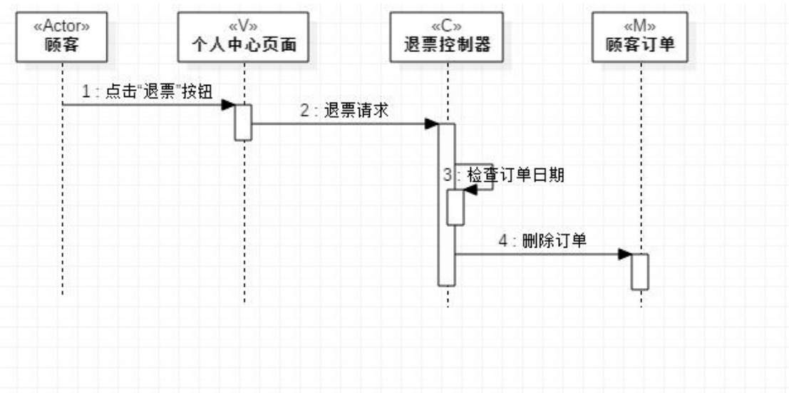
“退电影票”时序图
