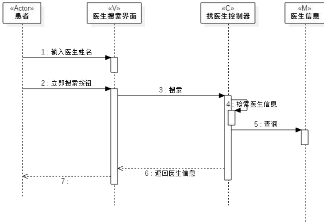
interaction SequenceDiagram1
